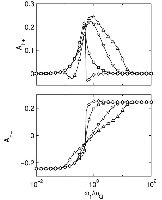
FIG. 7. As in Fig. 4, but for the \hat{T}_{31}(a) coherence [ g_{31}(t) ].
