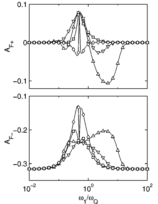
FIG. 8. As in Fig. 4, but for the \hat{T}_{33}(a) coherence [ g_{33}(t) ].
