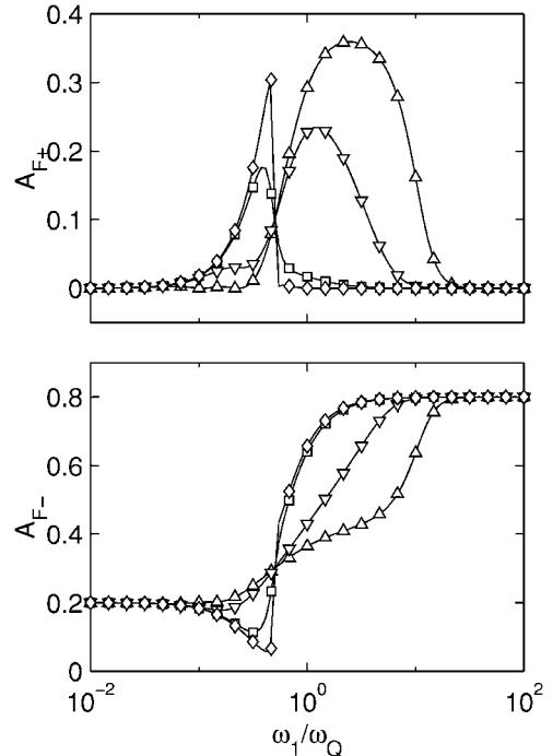
FIG. 4. Amplitudes of the fast modes (top) A_{F+} and (bottom) A_{F-} in the central resonance component of the \hat{T}_{11}(\alpha) coherence [g_{11}(t)] vs the relative RF field strength \omega_1/\omega_Q with a fixed scaled correlation time \omega_Q \tau_S = 0.1 . The symbols refer to the high frequency contributions to the spectral density: upper triangles, \alpha = 0.01 ; lower triangles, \alpha = 0.1 ; squares, \alpha = 1 ; and diamonds, \alpha = 10 .
