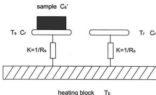
Fig. 1. Simplified DSC/MDSC cell with the temperature gradient in consideration, in the calculation, the cylindrical PET sample is equally divided into 10 small disks along its axis for finite element calculation. T_r is the reference temperature, T_s the measured sample temperature (or thermal couple temperature), C_r the heat capacity of the support plate, K=1/R_s is the system thermal constant.
