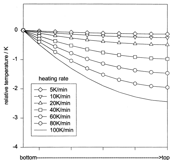
Fig. 5. Sample relative temperature distribution as a function of heating rate in conventional DSC by simulation. Sample bottom temperature is the reference point and set to zero.
