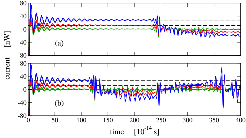
Figure 2.6: Plots of the current when the on-site spring constant is k_0 = 0.1 \text{ eV}/\text{\AA}^2\text{u} at 10% of the value of k_1 = 1 \text{ eV}/\text{\AA}^2\text{u} . The left and right chains have lengths (a) N = 100 and (b) N = 50 . The average temperature between the chains are T = 100 \text{ K} (green (lowest gray) line), T = 300 \text{ K} (red (middle gray) line), and T = 500 \text{ K} (blue (upper gray) line). The temperature offset \alpha = 10\% . The dash lines are the values of the steady-state current, corresponding to T = 100 \text{ K} , 300 \text{ K} , and 500 \text{ K} , calculated independently from the Landauer-like formula.
